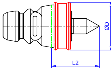
ADAPTOR TYPE SCCD.../60° DEAD CENTER.
