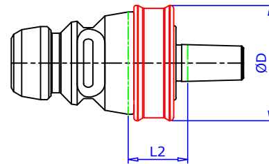
ADAPTOR TYPE SCDC.../B
