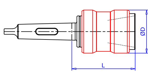
CHUCK TYPE SCDTC../ISO
